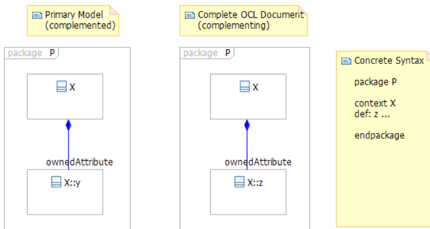
Figure 6: The Multiple Models problem for Complete OCL.
