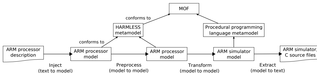
Figure 12: Simulator generation from HARMLESS models
