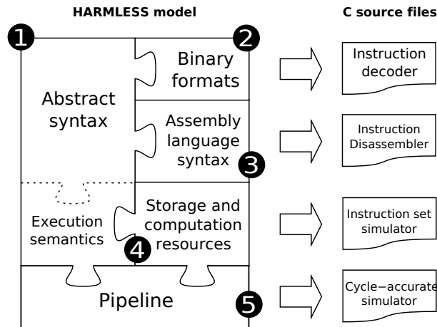
Figure 1: Processor views and simulator generation using HARMLESS
