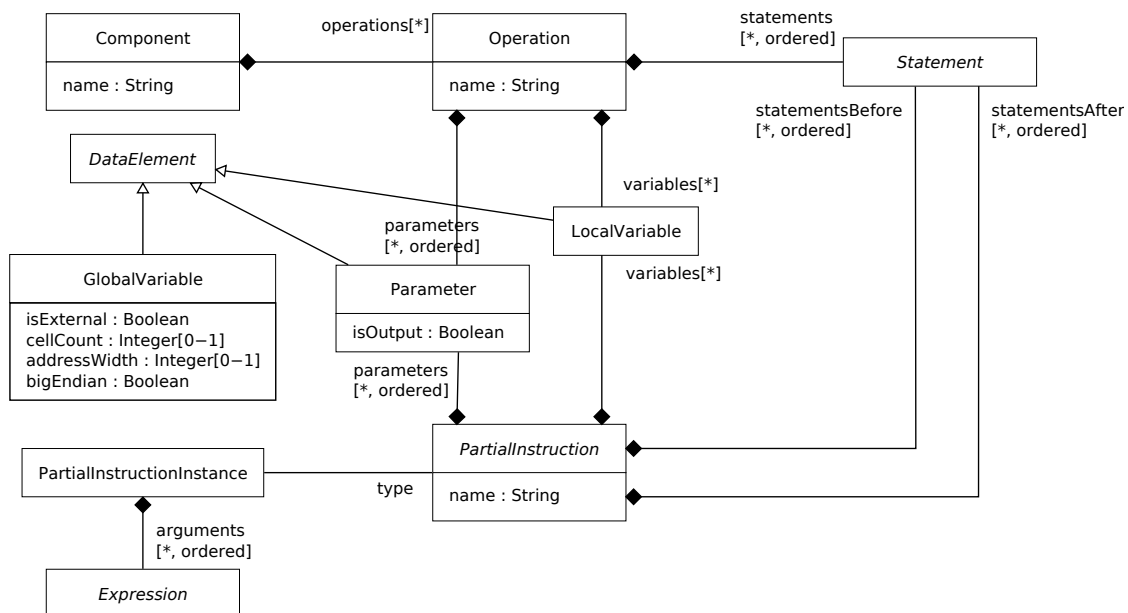
Figure 8: Extract of the HARMLESS metamodel: execution semantics of partial instructions
