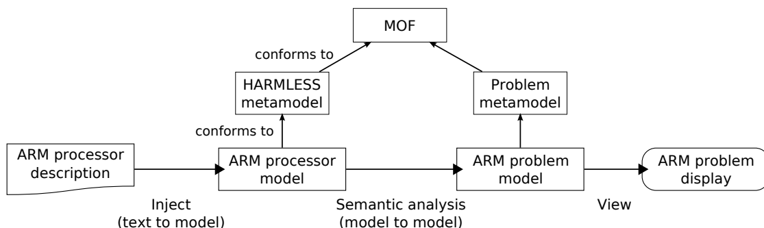
Figure 11: Semantic analysis of HARMLESS models and error reporting
